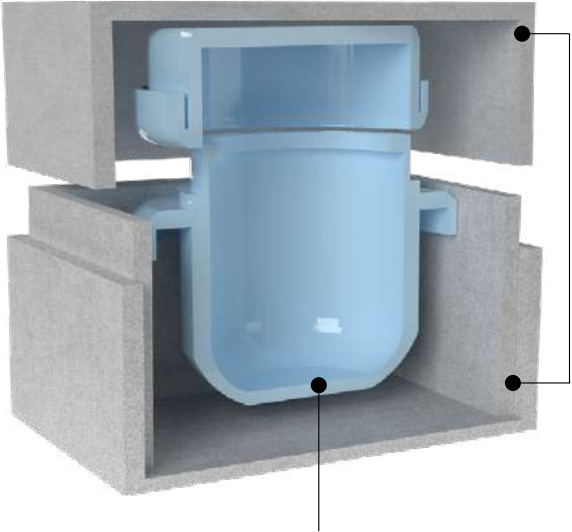
outer container Material: 23g Paper rebo paper jar 50ml as an example
