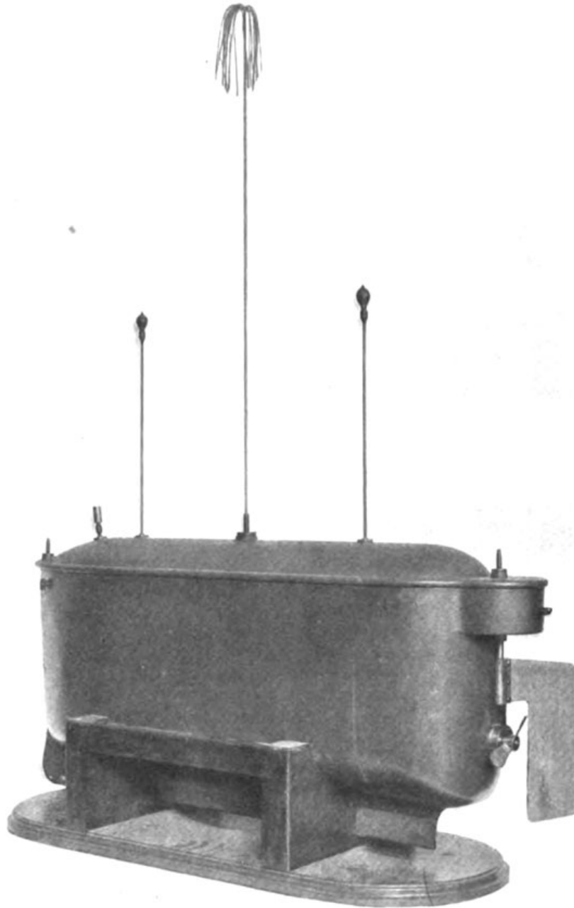
FIG. 2. THE FIRST PRACTICAL TELAUTOMATON.
