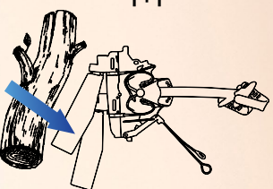
Kick-Up Fins Retract When Impacting an Underwater Obstacle
