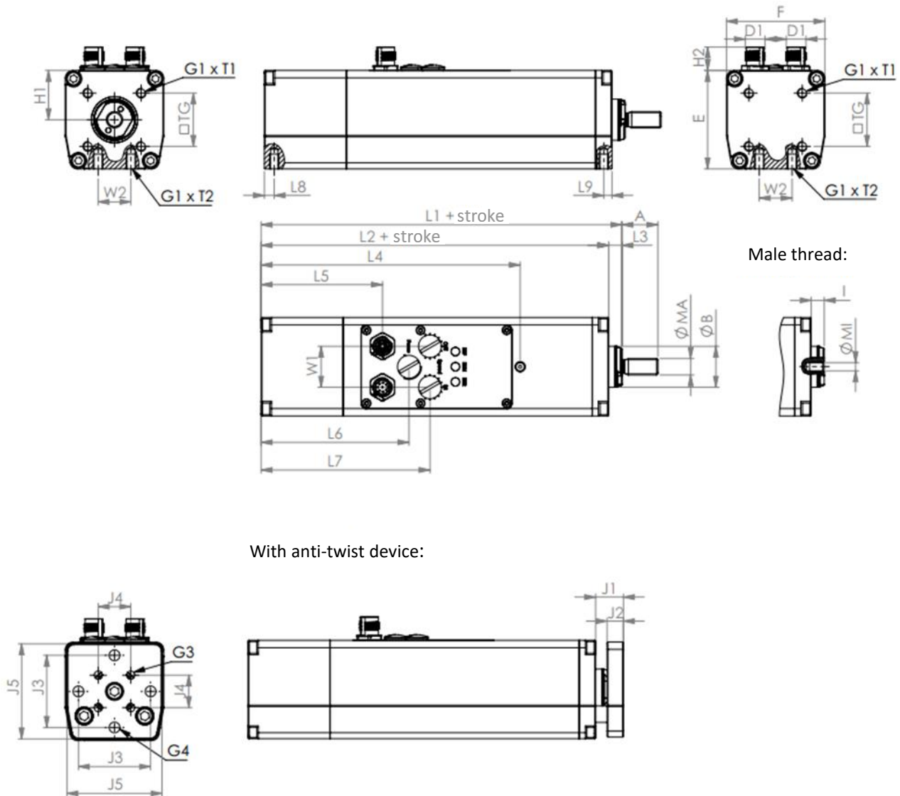
FIGURE 4: DIMENSIONS
