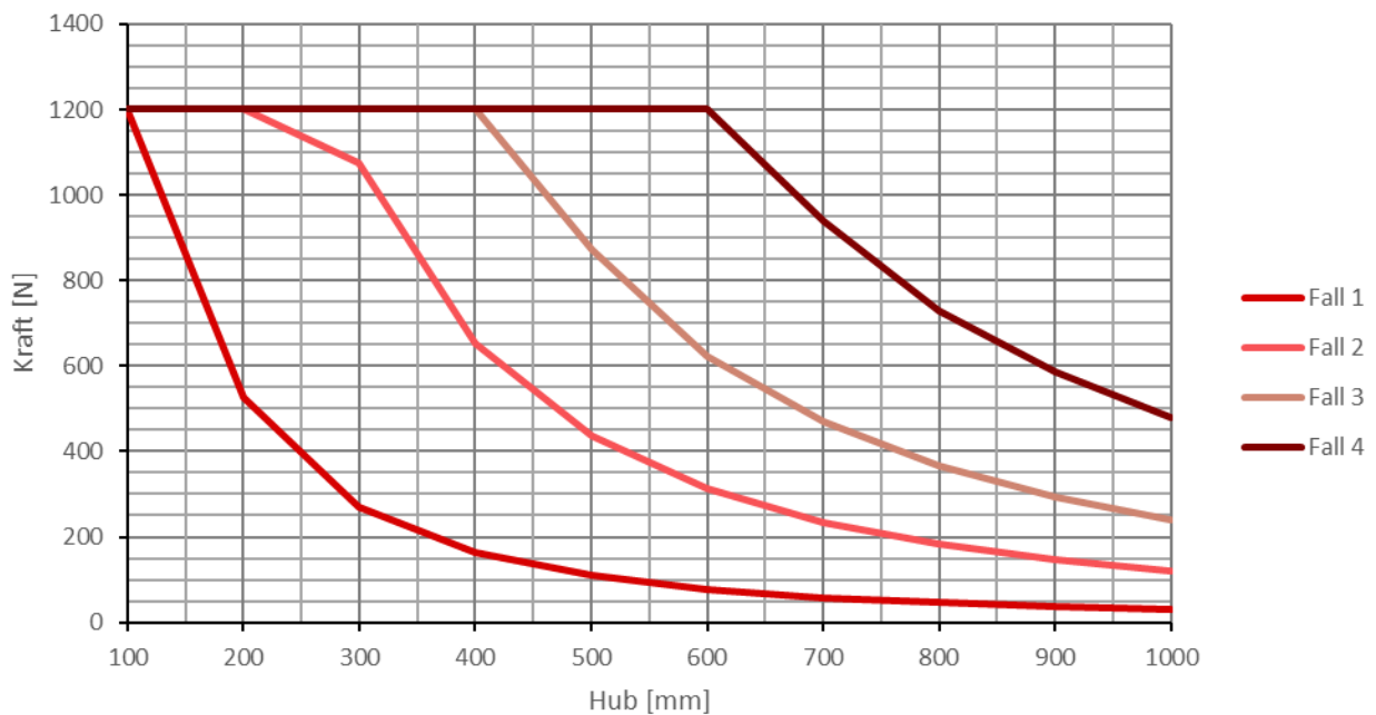
Permissible compressive force according to installation case
