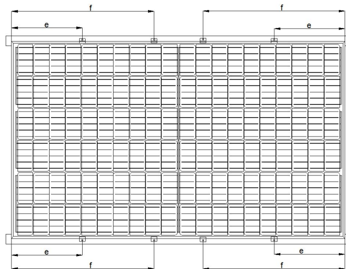
Figure 5: 209mm < e < 259mm、729mm < f < 779mm
