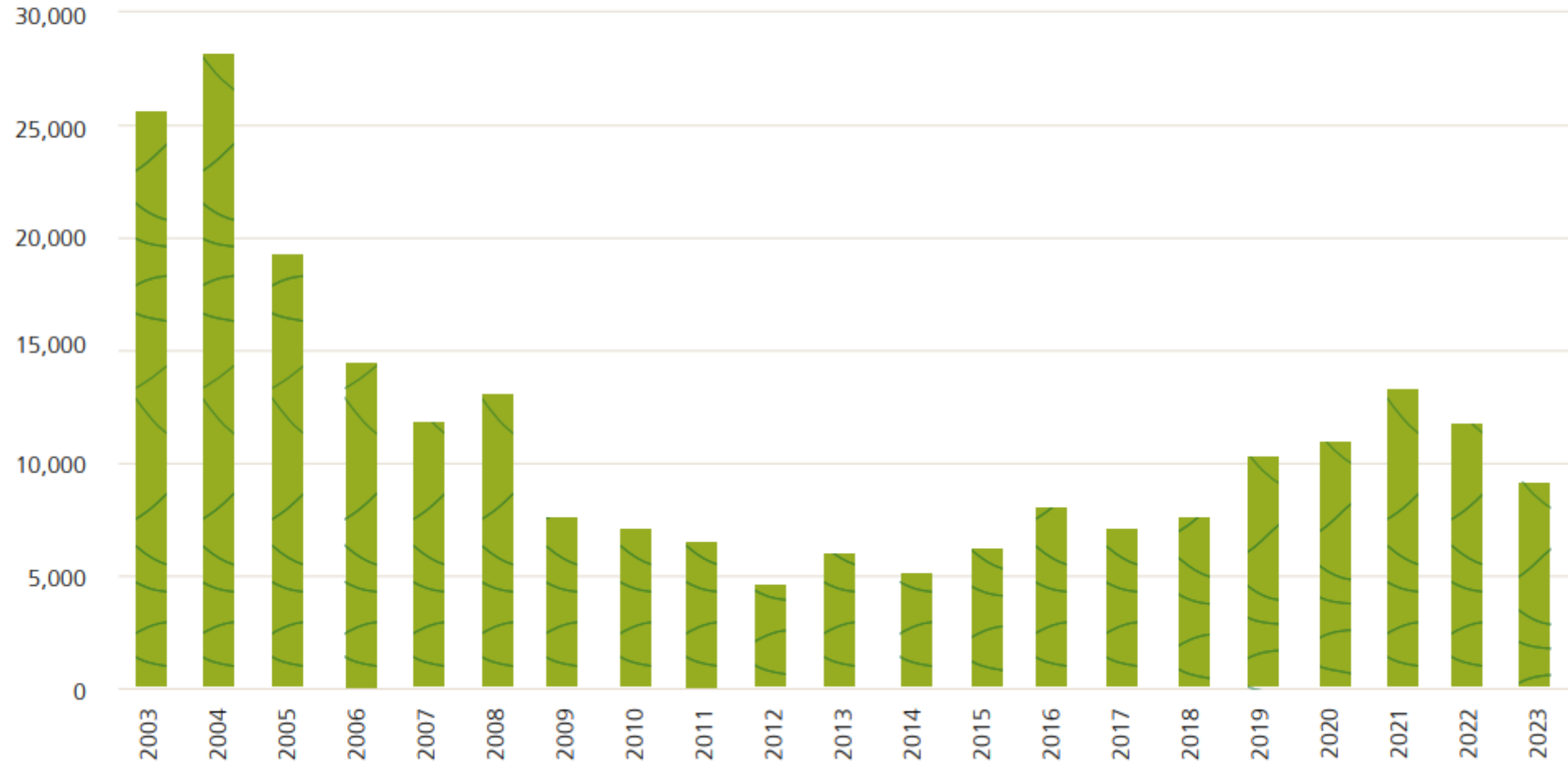
GRAPH 2 | ANNUAL DEFORESTATION IN THE LEGAL AMAZON BY CLEAR CUTTING (KM 2 ) *
