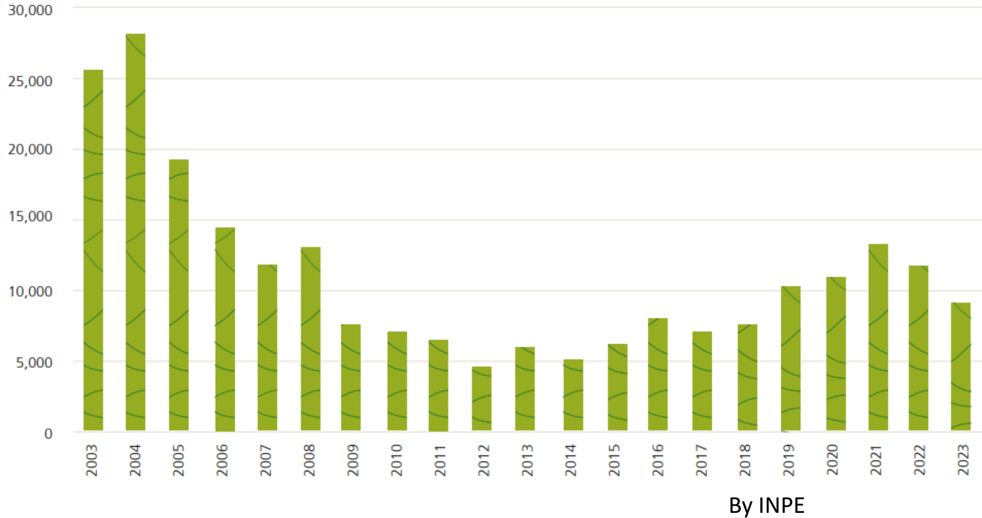
GRAPH 2 | ANNUAL DEFORESTATION IN THE LEGAL AMAZON BY CLEAR CUTTING (KM 2 ) *
