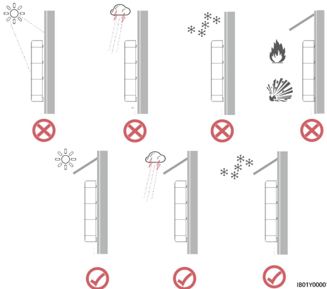
Abbildung 1-3 Installation environment
