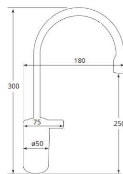
T3 3-way column tap
