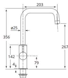
T5 5-way tap - 2 ways for hot and cold unfiltered water and 3 for filtered water
