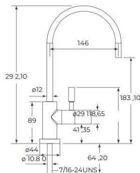
T1 1-way tap
