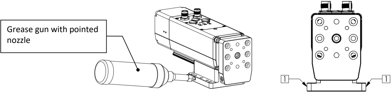
FIGURE 10: RELUBRICATION OF LINEAR GUIDE FOR CTC-060-K__-____-F
