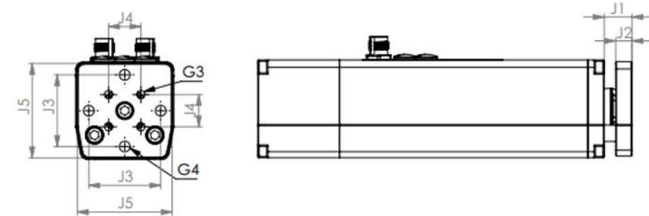
FIGURE 4: DIMENSIONS
