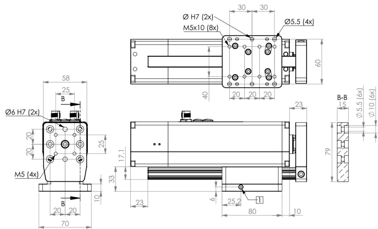
FIGURE 5: DIMENSIONS CTC-060-K__-____-F
