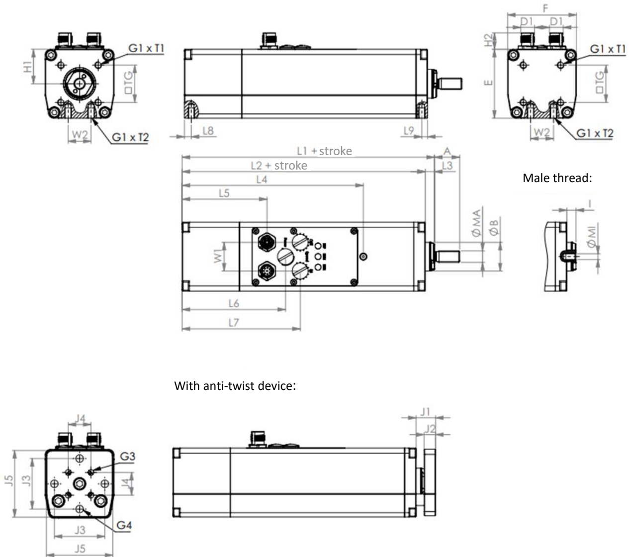
FIGURE 4: DIMENSIONS
