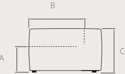
A Seat height 41cm B Seat depth 70cm C Height 64cm
